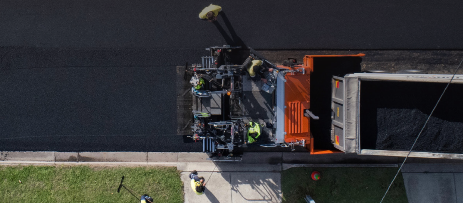
Paving low temperature Gap Graded Asphalt with crumb rubber
