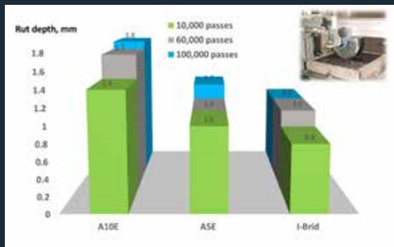
Typical wheel tracking performance @ 65°C of AC14 with different high-performance binders
